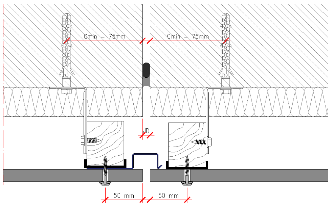
Figure 2.1.40 - Expansion joint
