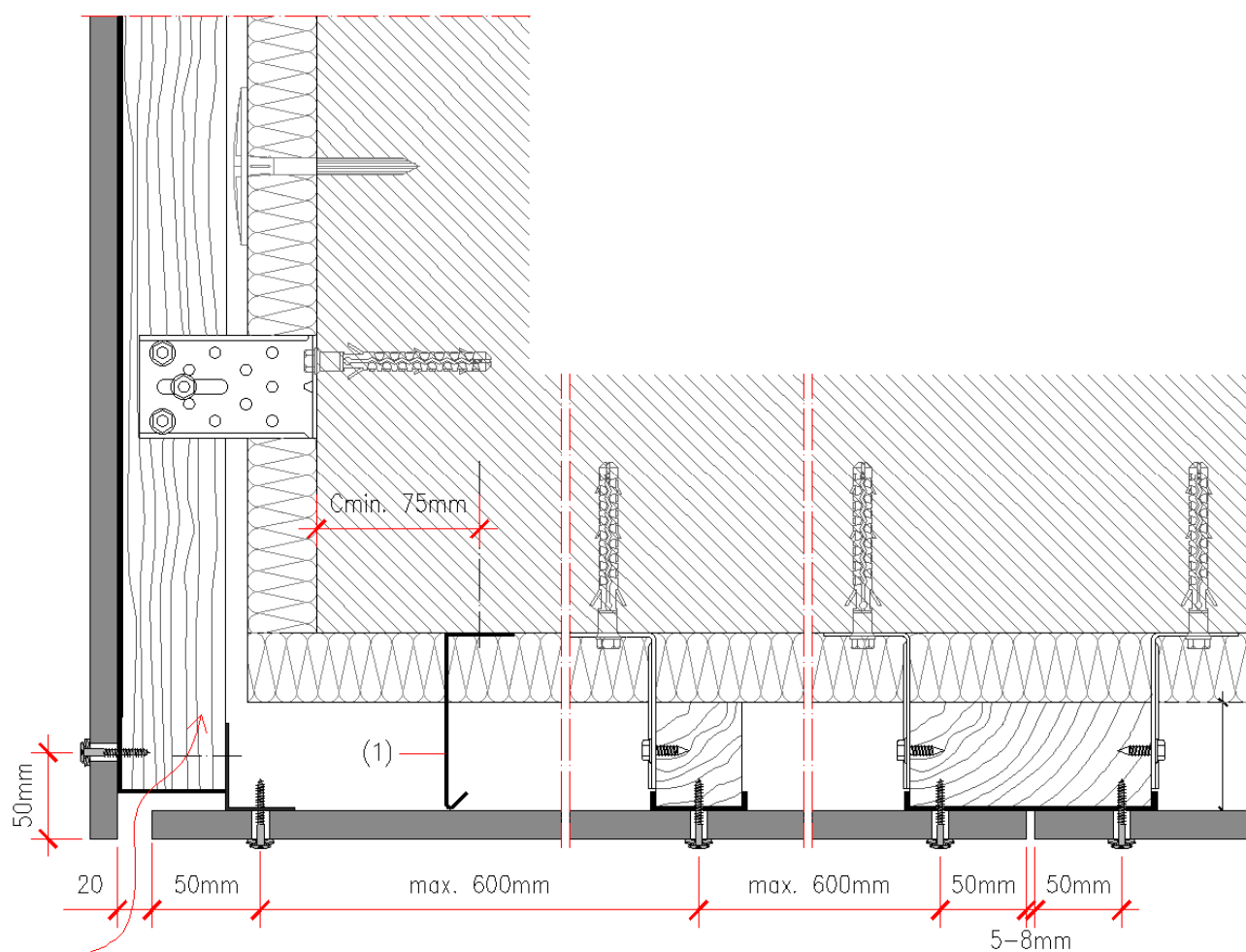
Figure 2.1.50 - Detail of the façade - false ceiling connection
