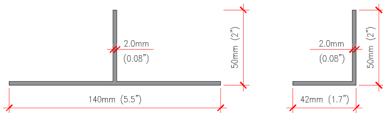
Figure 2.1.4 - Aluminium structure 6000 series alloy with R_{p0.2} \geq 180 \text{ MPa}
