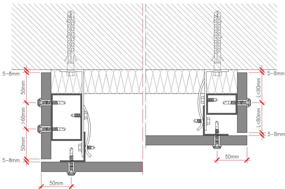
Figure 2.1.70 - Side finish
