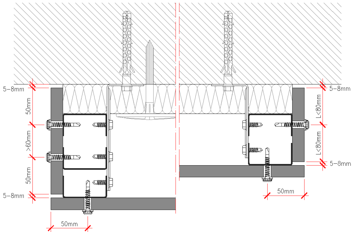
Figure 2.1.54 - Side finish
