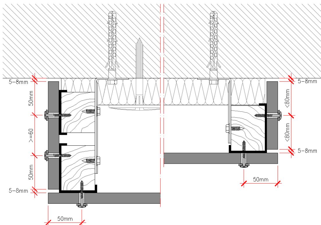
Figure 2.1.39 - Side finish
