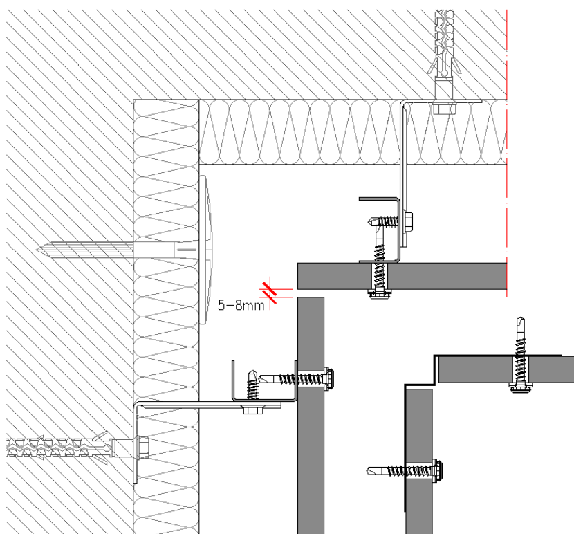
Figure 2.156 - Corner angle
