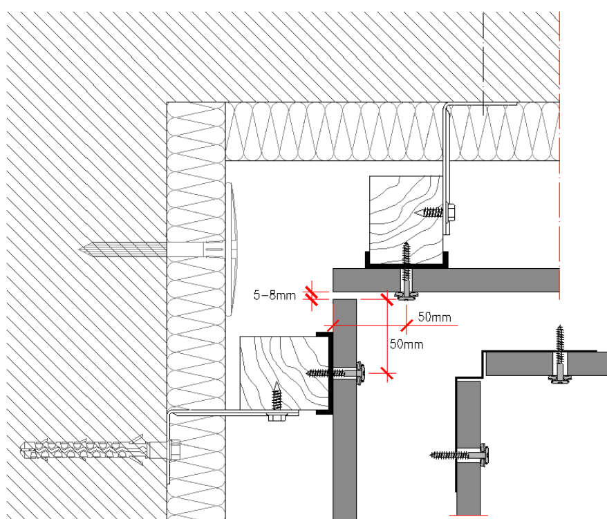
Figure 2.1.41 - Corner angle
