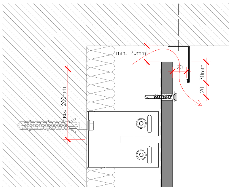
Figure 2.1.69 - Balcony finish
