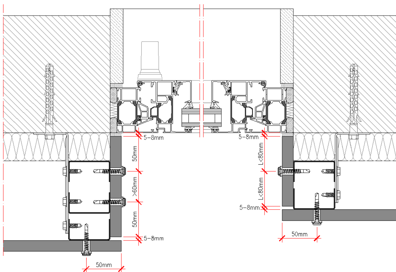
Figure 2.1.61 - Horizontal section, window opening
