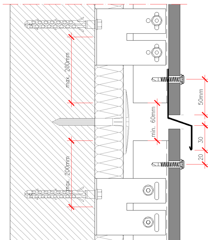
Figure 2.1.81 - Fractionation of the structure: Profiles length > 6 m
