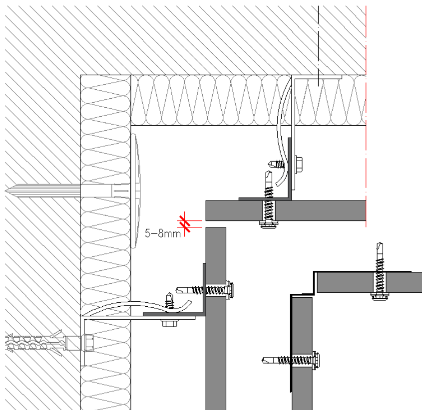
Figure 2.1.72 - Corner angle
