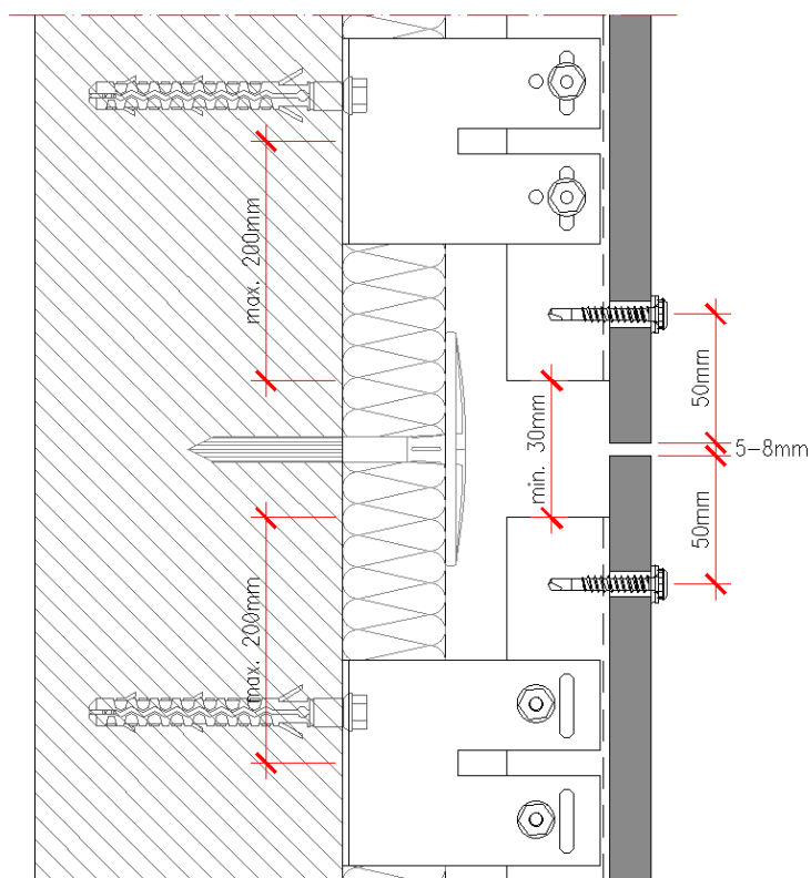
Figure 2.1.80 - Fractionation of the structure: Profiles length \leq 6 m
