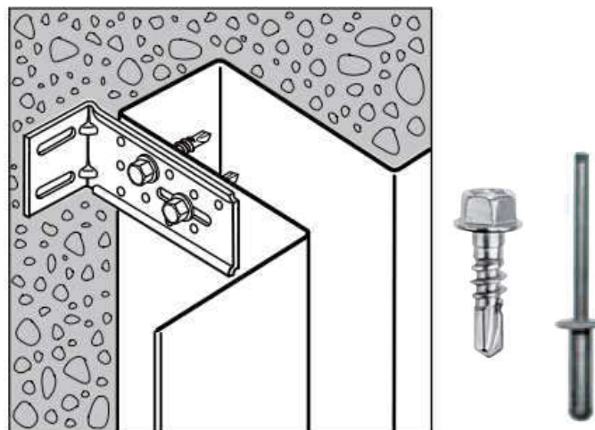
Figure 2.3.15 - Fixing the galvanised steel profiles to the supporting squares ( \varnothing \geq 5.5 screws or \varnothing \geq 4.8 rivets)
